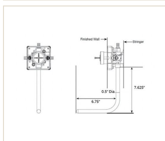
Universal Valve with Copper Tub Spout AX-PBV-1002
