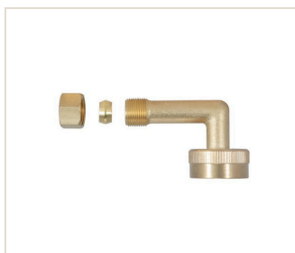
Dishwasher Connector AX-PP-YD1007 Dishwasher Connector; 3/8" Comp x 3/4" FHT Elbows
