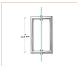
Mitered Corner Back-to-Back Pull Handle AX-GEH2-PD8 Polished Chrome 8" Round Tubing; Mitered Corner Back-to-Back Pull Handle
