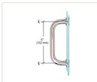
Single-Sided Pull Handle AX-GEH1-PS6 Polished Chrome 6" Tubular; Single-Sided Pull Handle
