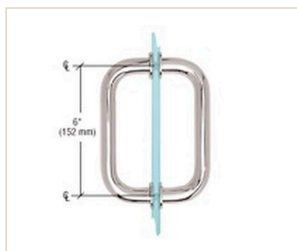
Back-to-Back Pull Handle AX-GEH1-PD6 Polished Chrome 6" Tubular; Back-to-Back Pull Handle
