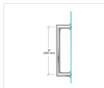
Mitered Corner Single Sided Pull Handle AX-GEH2-PS8 Polished Chrome 8" Round Tubing; Mitered Corner Single Sided Pull Handle
