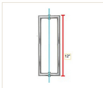
Mitered Corner Back-to-Back Pull Handle AX-GEH2-PD12 Polished Chrome 12" Round Tubing; Mitered Corner Back-to-Back Pull Handle
