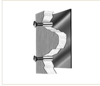
Installation Hardware AX-BHC-1464
